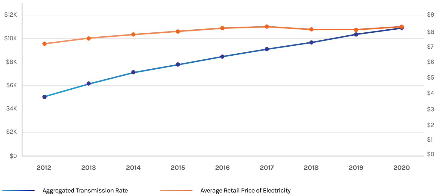
Fig.2 Regional Aggregated Transmission Rates vs Average Retail Price of Electricity
